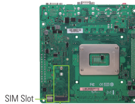
M.2 Key B ▲ Rear view (2242/3042/3052)
